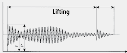
Example of dynamic chain loading in the hoist during the lifting cycle
